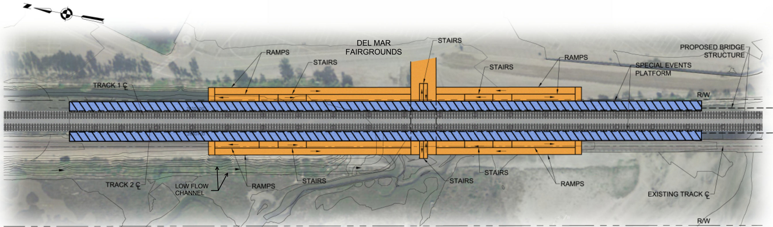
SIDE LOADING PLATFORM PLAN
