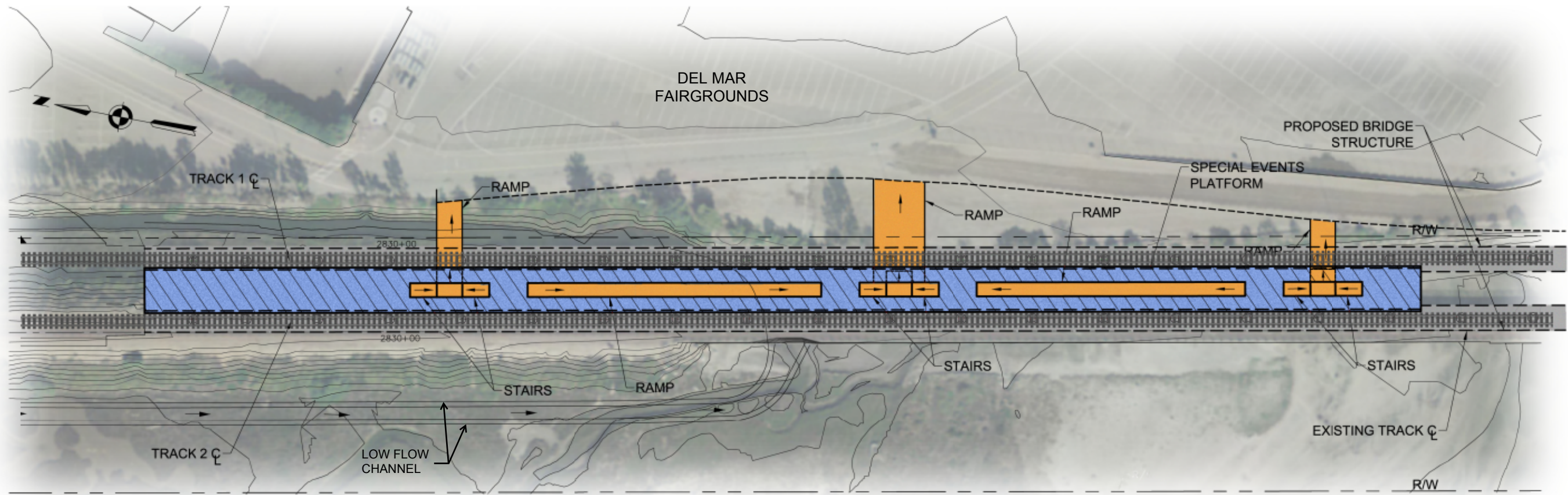
CENTER LOADING PLATFORM PLAN
