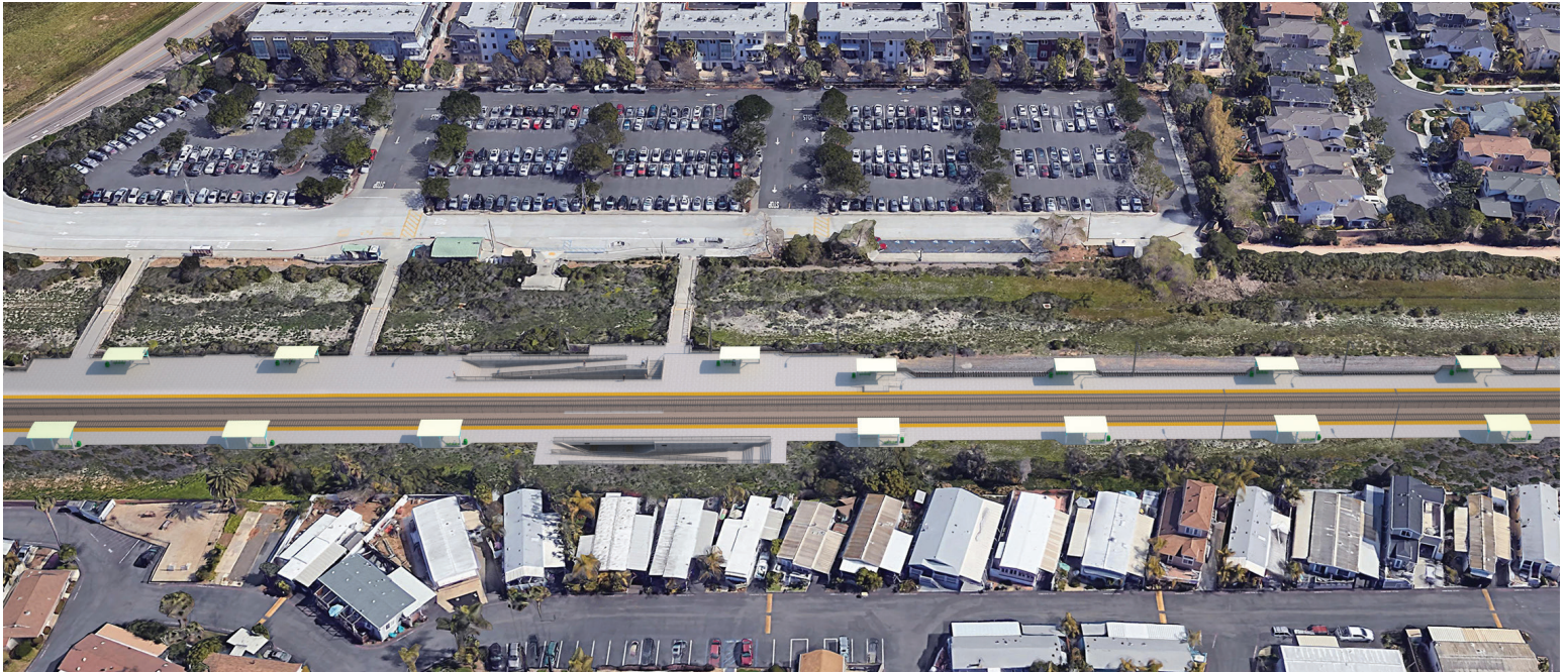
Visual simulation of planned platform improvements: looking east
