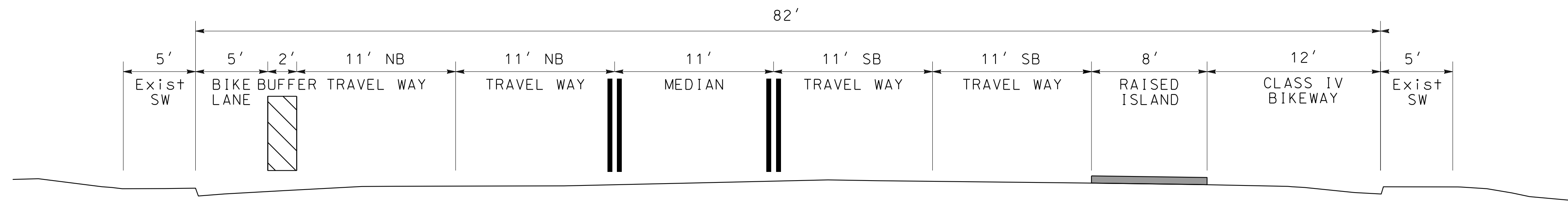
J-J: PROPOSED BIKEWAY ON BEYER BLVD (CLASS II & IV) IRIS AVE TO DAIRY MART RD
