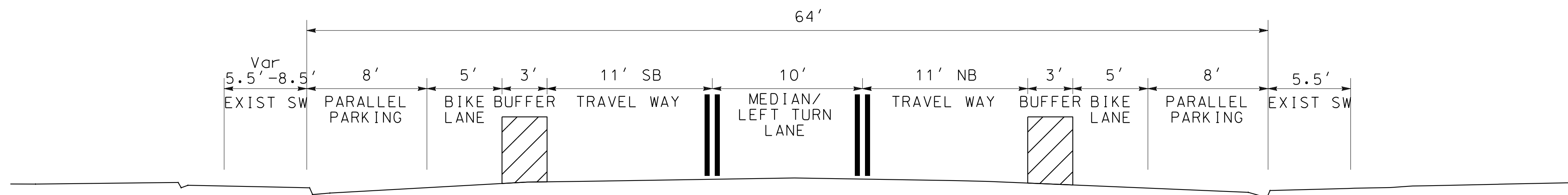
B-B: PROPOSED BIKEWAY ON 13th St (CLASS II) DONAX Ave TO EBONY Ave FERN Ave TO GROVE Ave
