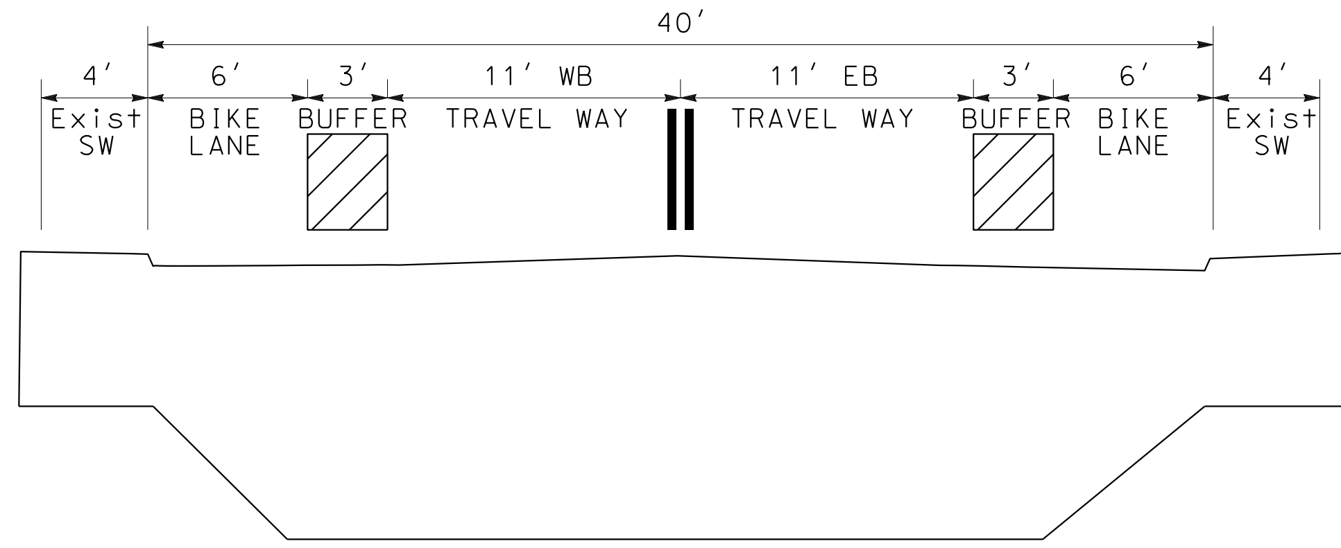
G-G: PROPOSED BIKEWAY ON IRIS AVE (CLASS II) EXISTING BRIDGE OVER FREEWAY
