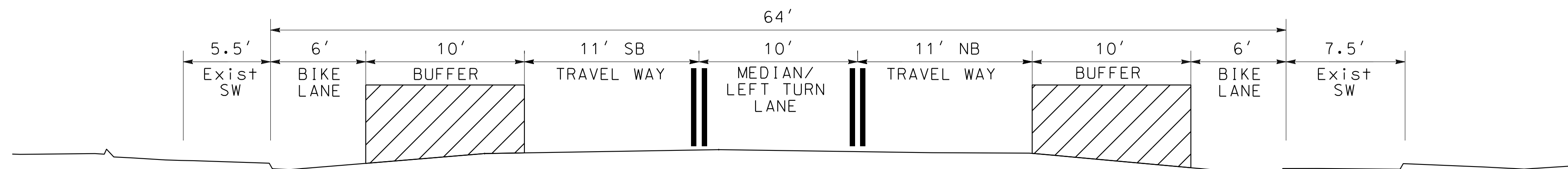
C-C: PROPOSED BIKEWAY ON 13TH ST (CLASS II) EBONY Ave TO FERN Ave
