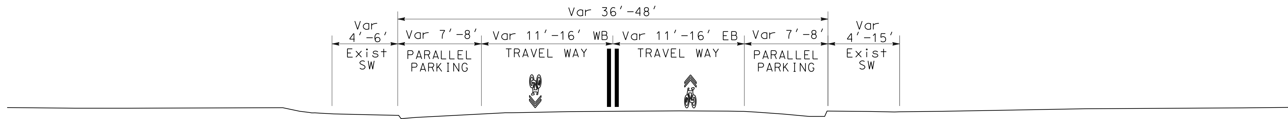
D-D: PROPOSED BIKEWAY ON GROVE AVE (CLASS III) 13th St TO WEST OF SATURN Blvd SWITZERLAND Dr TO ORO VISTA Rd
