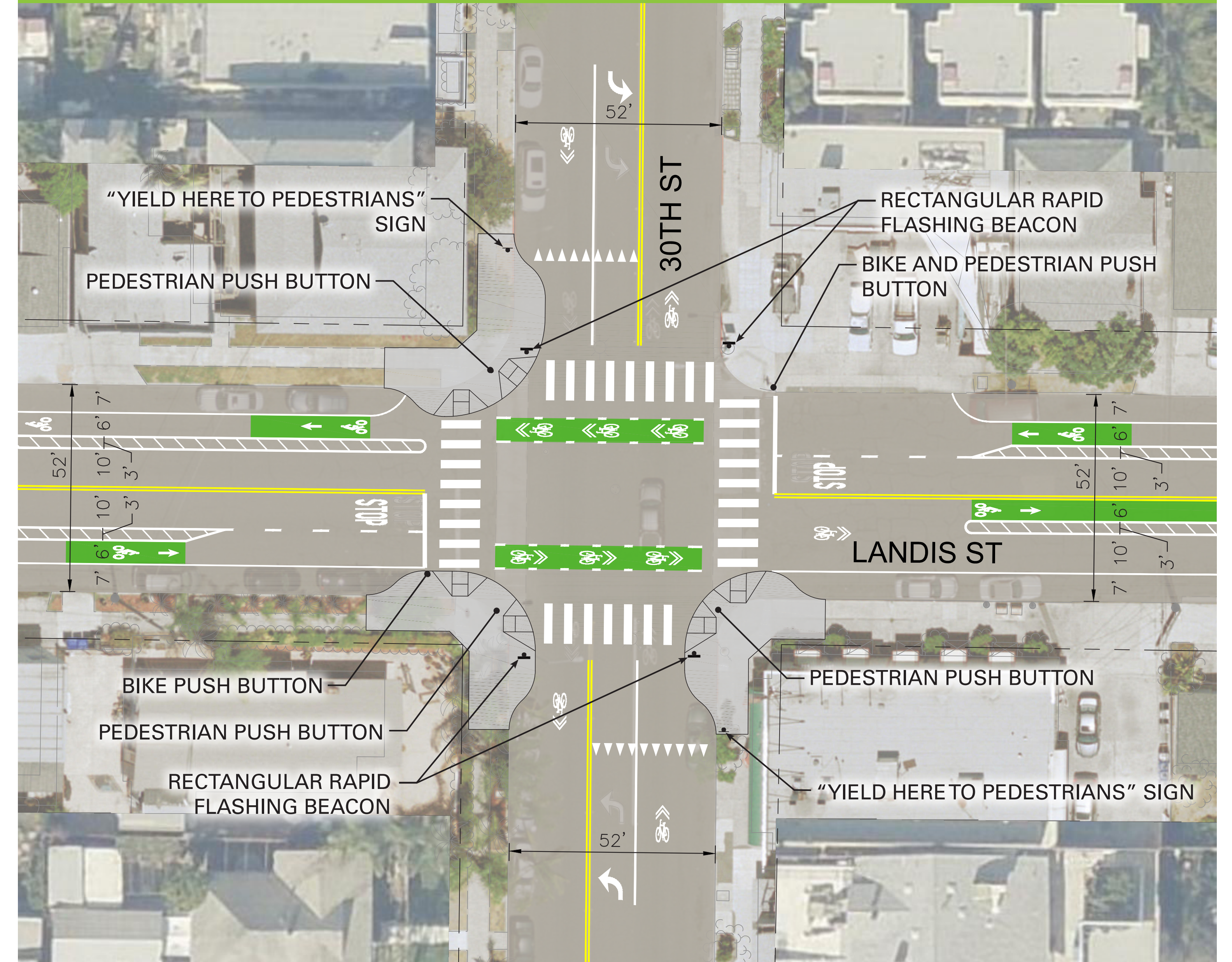
Landis and 30th - Rectangular Rapid Flashing Beacon
