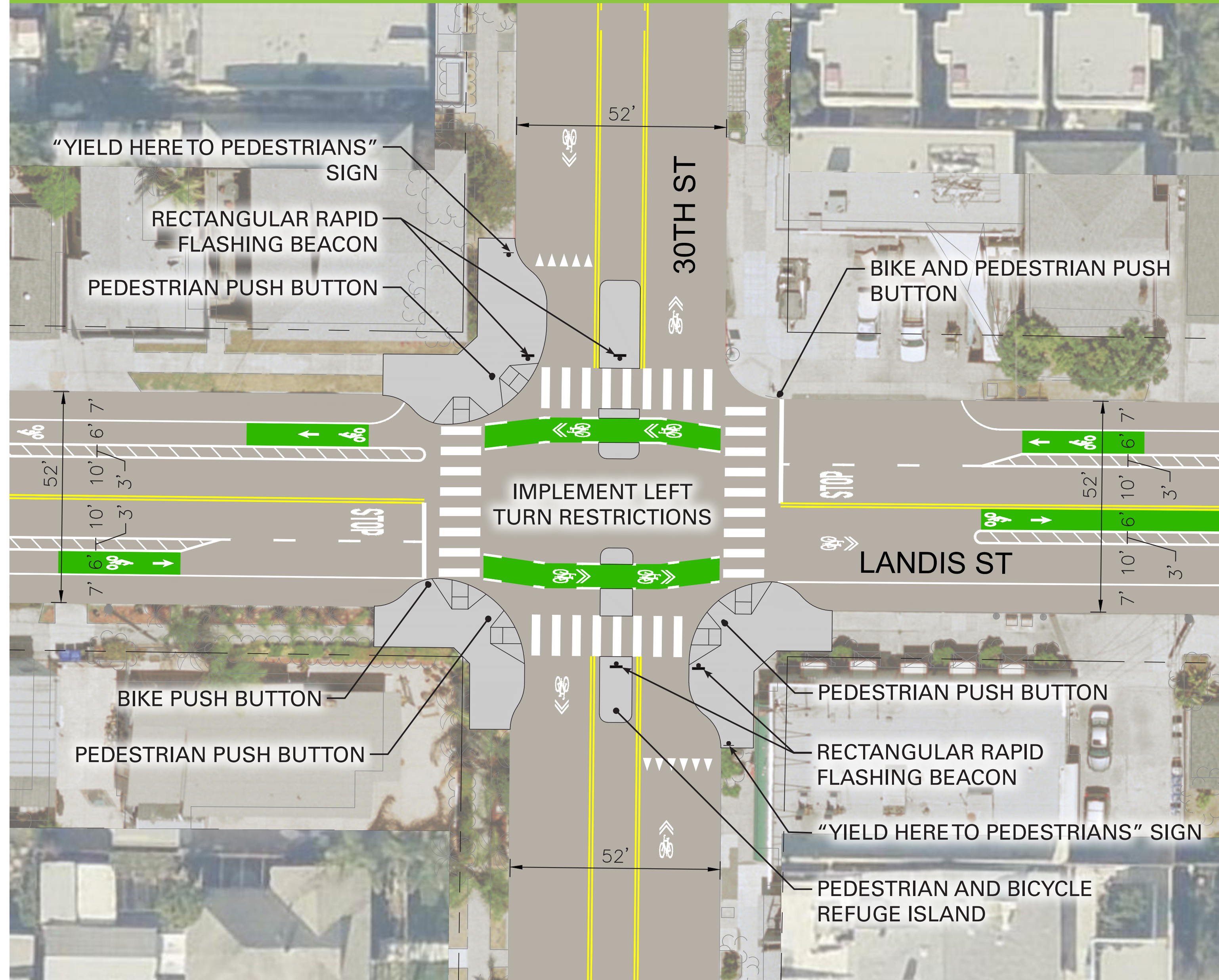
Landis and 30th - Rectangular Rapid Flashing Beacon with Refuge Island
